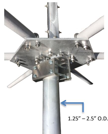
Universal mast fixture
