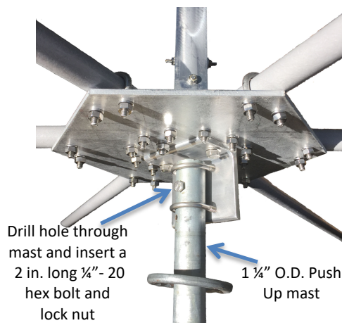
Standard mast fixture
